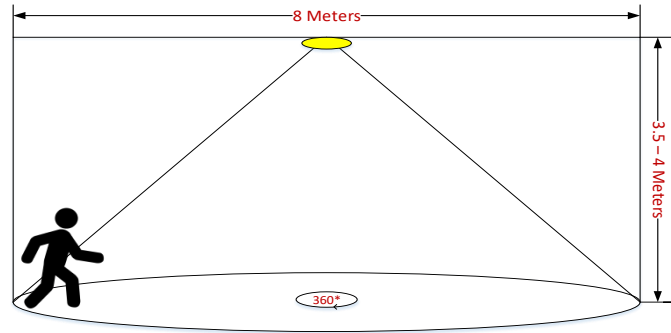
Tulip Sensor Light Motion Detection Range
